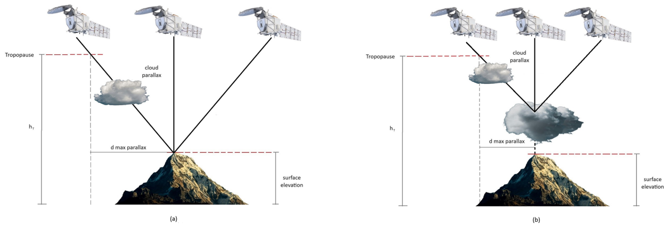
Figure 2. Diagram illustrating the presence of cloud parallax in a co-registered fore observation under nadir-observed clear-sky (a) and cloudy conditions (b). Satellite image provided courtesy of ESA.
