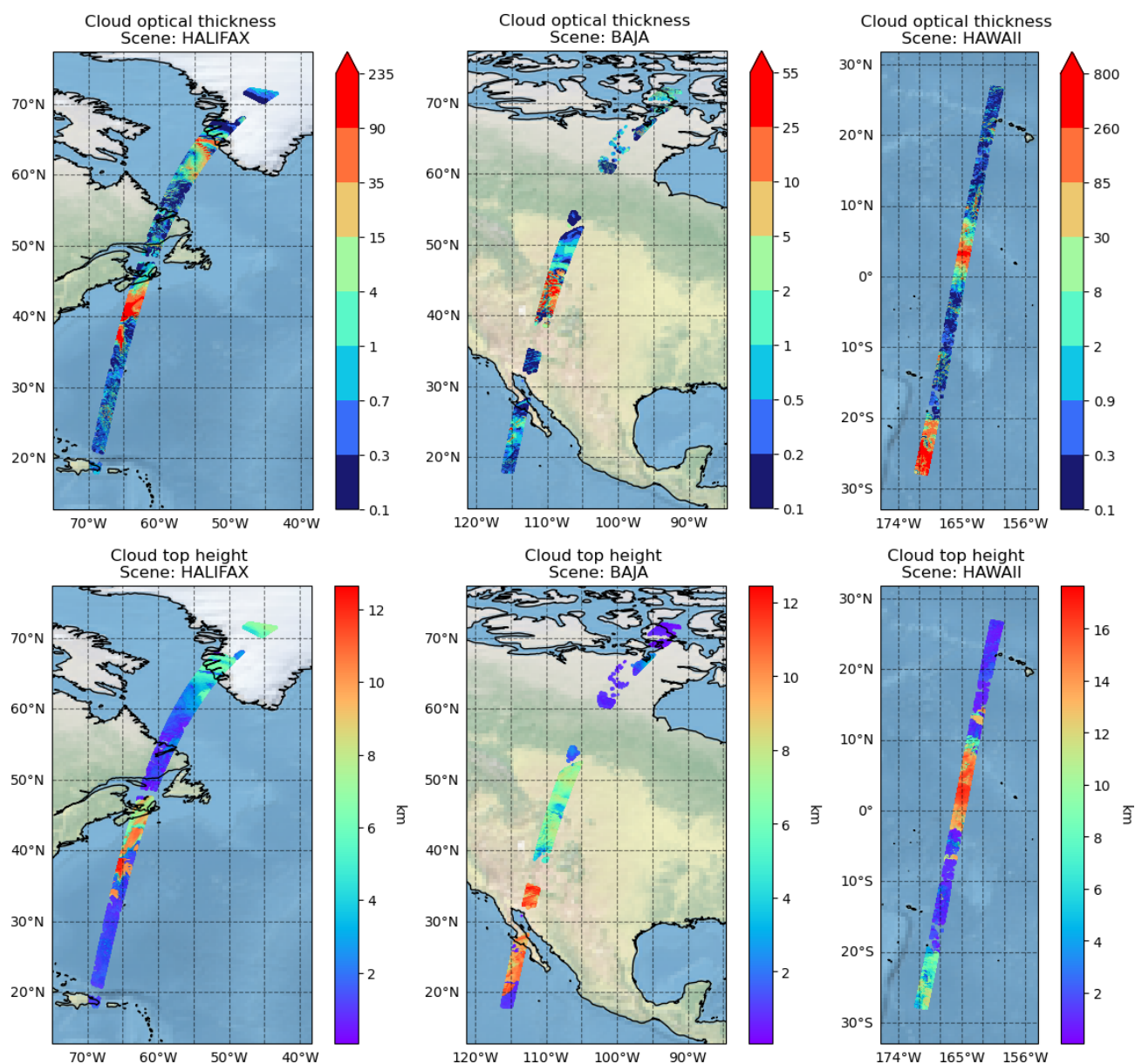
Figure 3. MSI-like model truth cloud optical thickness and cloud top height for the three scenes. Colour bars ending with an arrow are logarithmic and have cloud optical thickness values greater than the upper tick label plotted in red. The cloud properties have been calculated using a COT threshold of 0.1.
