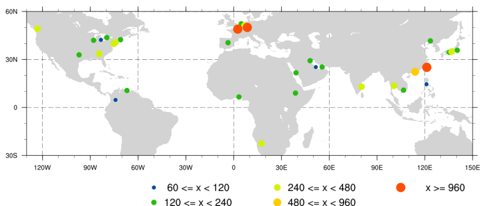
Figure 1. Locations of the 33 selected airports with IAGOS data for the 2008–2020 period. The sizes of the symbols are proportional to the number of valid profiles used for validation.
