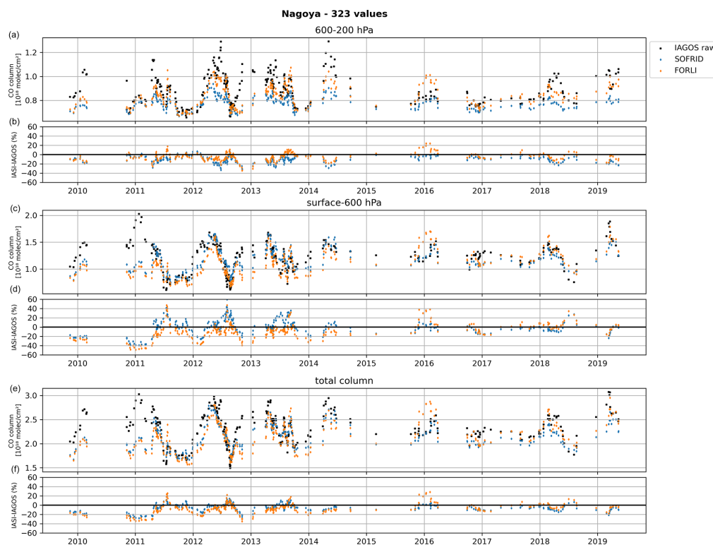
Figure 11. Same as Fig. 7 but for Nagoya.
