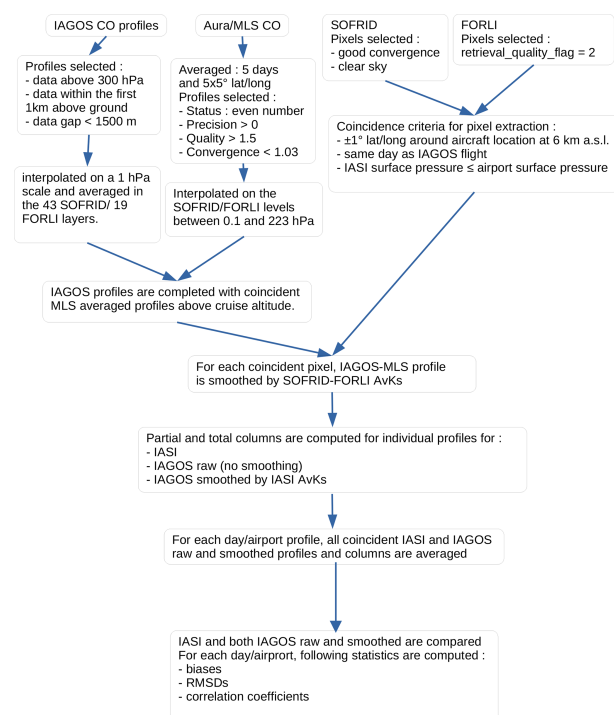
Figure 4. Flowchart of the validation methodology.
