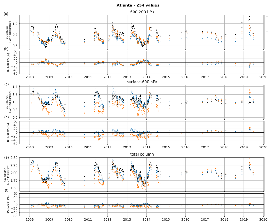
Figure 8. Same as Fig. 7 but for Atlanta.
