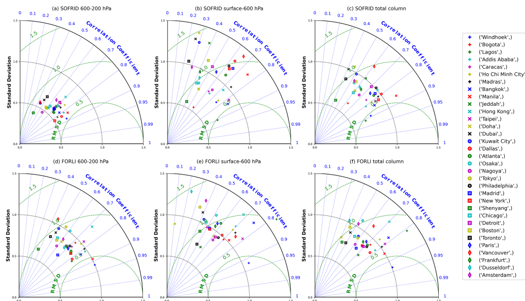
Figure A1. Taylor diagrams for the SOFRID (a–c) and FORLI (d–f) versus IAGOS smoothed data comparisons for the 600–200 hPa (a, d), surface–600 hPa (b, e) and total (c, f) CO columns.
