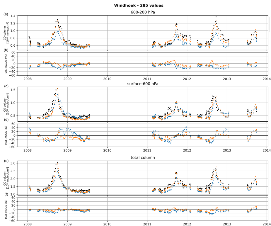
Figure 12. Same as Fig. 7 but for Windhoek.
